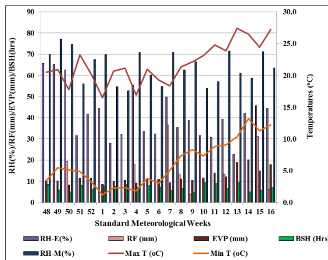
Fig 1: Climatograph of the study area for crop growing period
